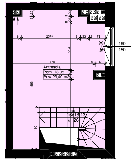
ANTRESOLA
