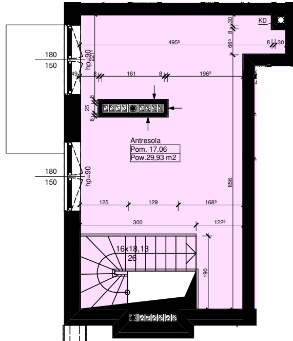
ANTRESOLA
