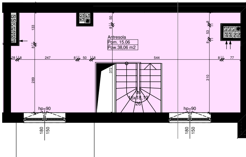
ANTRESOLA
